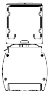
P2000 Hanger Bracket
